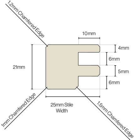
Brooklyn Stile Cross Section
